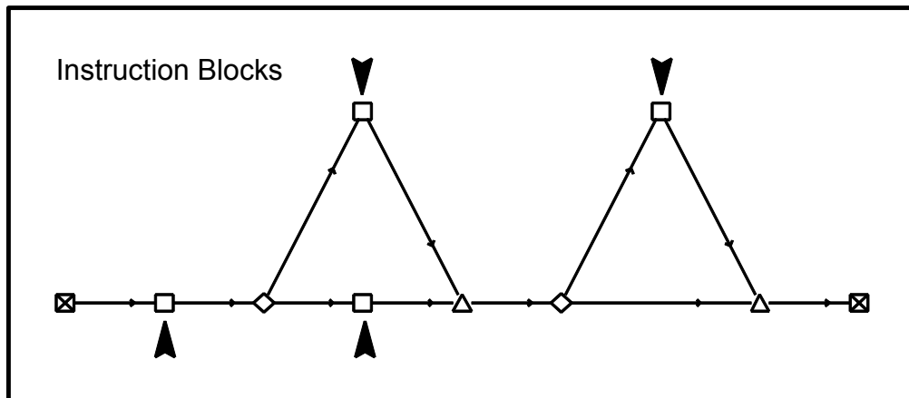
Control graph with 4 IBs
