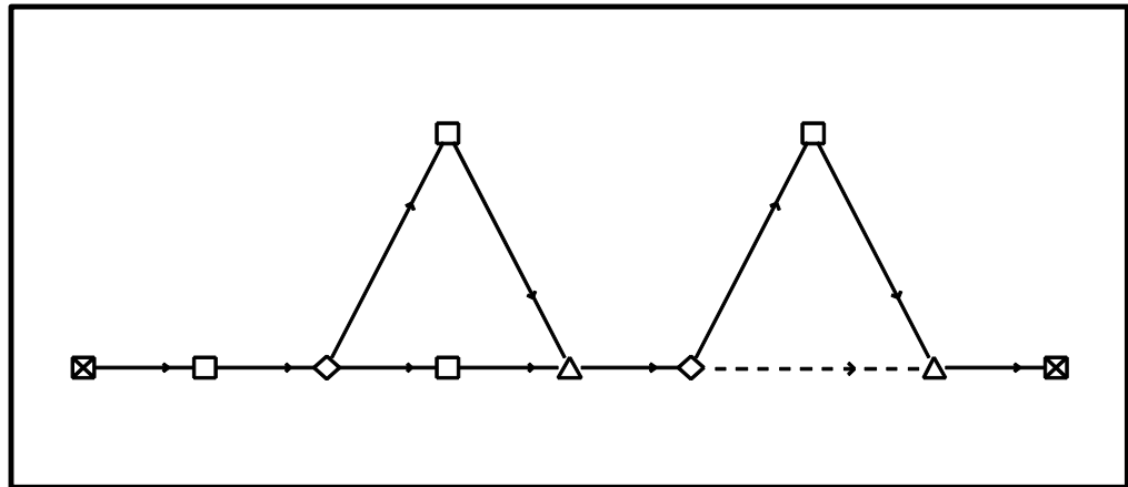
Control graph of paths taken
