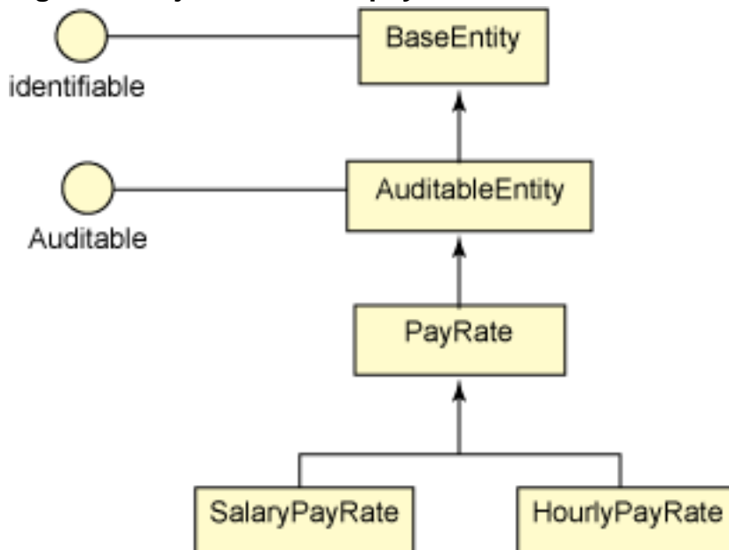
Figure 1. Object model for pay-rate calculations
