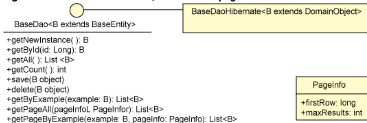
Figure 3. The BaseDao interface, extended for pagination
