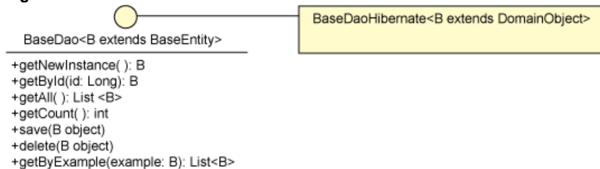
Figure 2. The extended BaseDao interface
